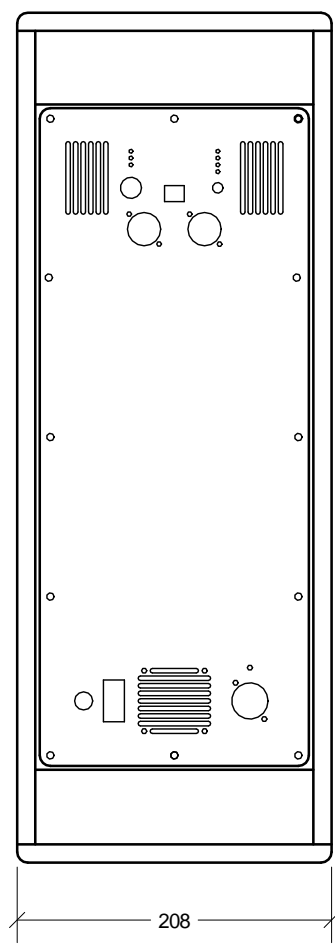
REAR ELEVATION
