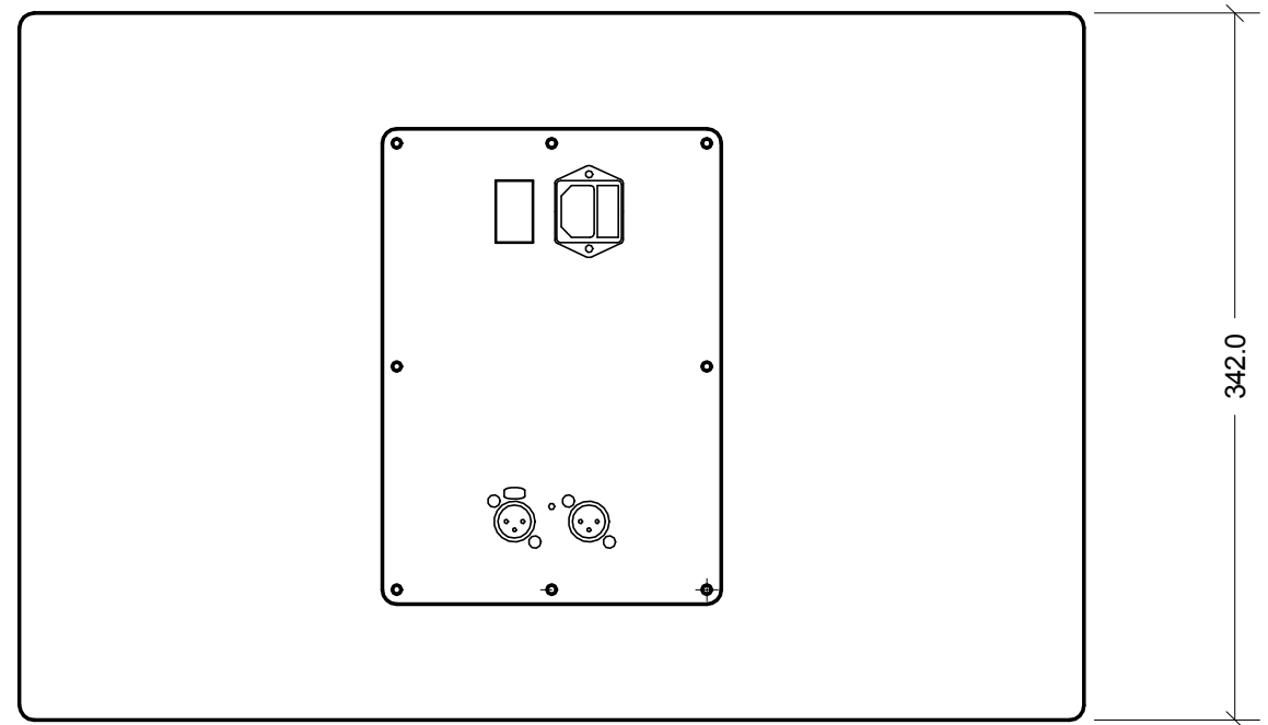
REAR ELEVATION
